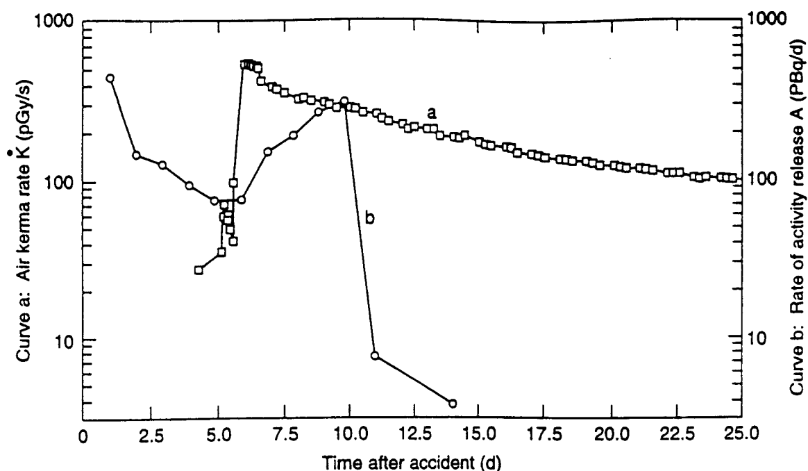
Figure 2. Measurements of the air kerma rate (curve a) and the activity release rate (curve b) made at the reference point located at the Vinca Institute during the active Chernobyl accident phase (24).
