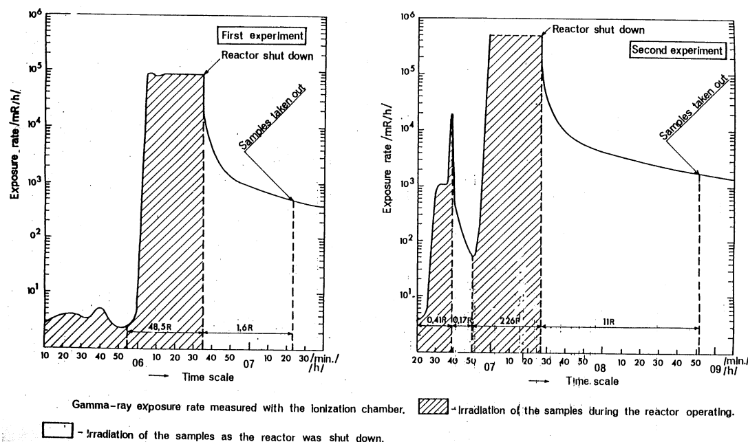
Figure 1. Exposure dose intensity, measured by a KAKTUS ionization chamber, during intercomparison experiments at the RB reactor.
